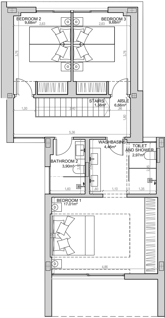
TOP FLOOR
