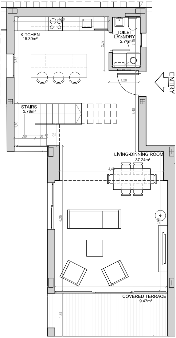
GROUND FLOOR
